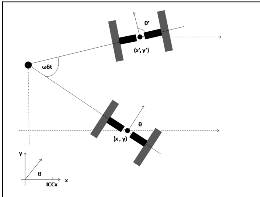
Rotating the robot \omega \delta t degrees around the ICC
