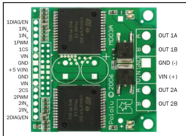
Dual VN12SP30 motor driver carrier MD03A
