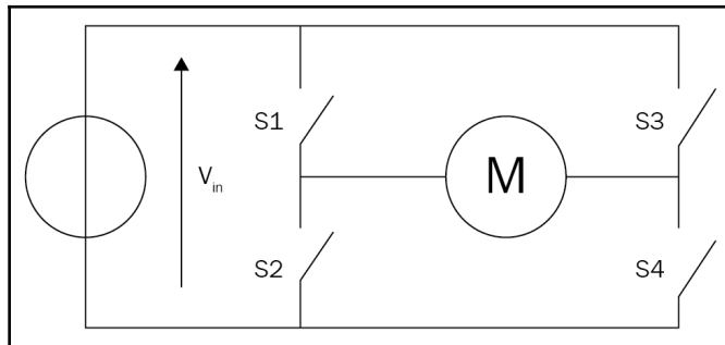
H-bridge circuit
