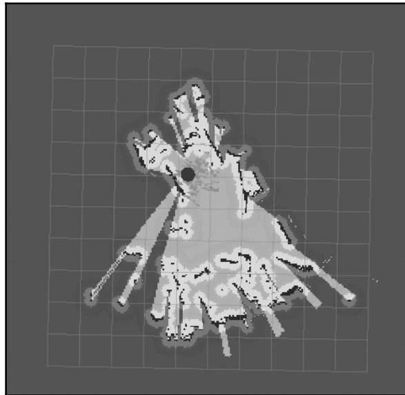
Localizing the robot using AMCL
