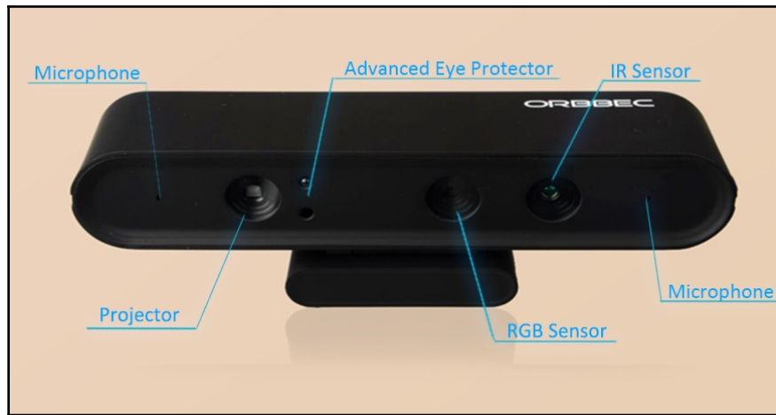
Orbbec Astra depth sensor ( https://orbbec3d.com/product-astra/ )
