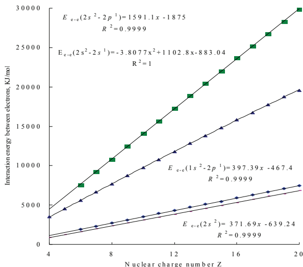
Figure 5.3. The relationship between the interaction energy of the electrons in 2 nd layers and the nuclear charge number.
