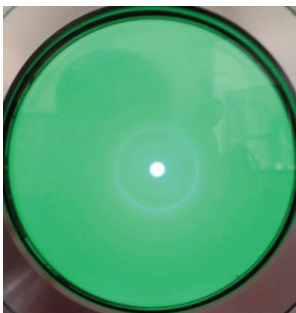
Figure 2.4. Electron diffraction pattern (unaffected by magnetic field).
