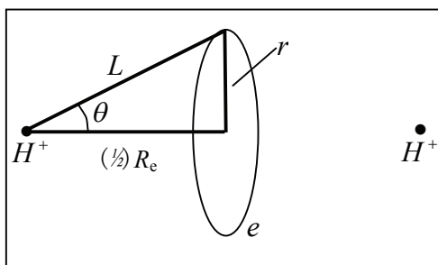
Figure 4.2. Hydrogen molecule-ion
