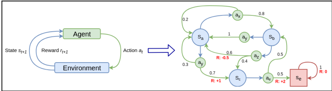
Left: The agent takes an action and receives the new state and reward. Right: An example of a simple MDP with four states ( s_a , s_b , s_c , and a terminal state, s_e ) and four actions ( a_x , a_y , a_z , and a_e ). Each action has a transition probability, but only some actions have rewards
