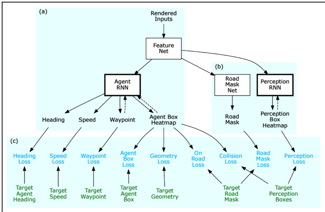
ChauffeurNet training components: (a) the model itself, (b) the additional networks, and (c) the losses (source: https://arxiv.org/abs/1812.03079 )
