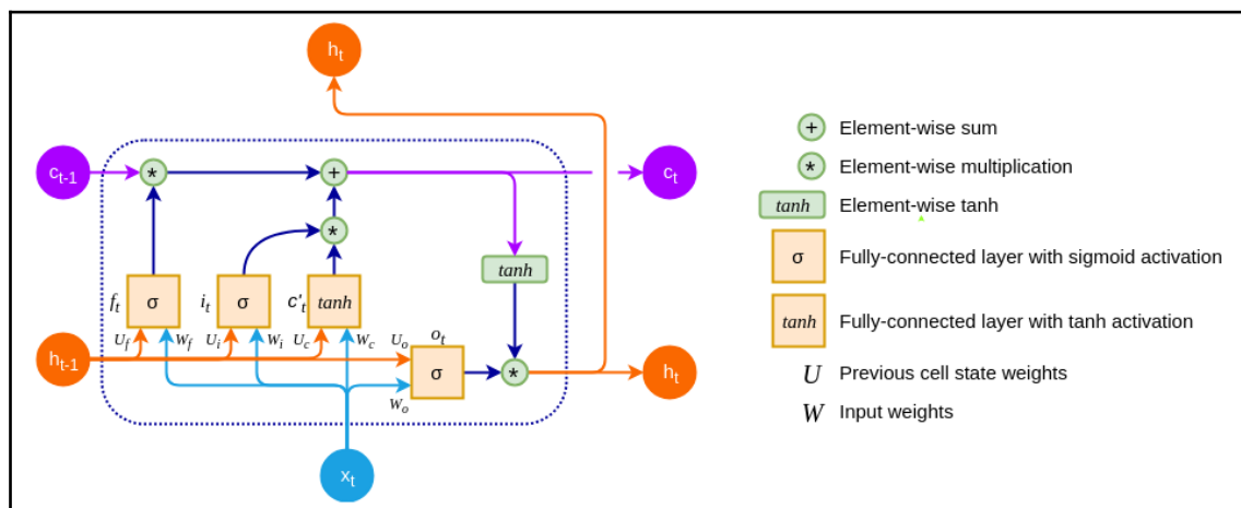
LSTM cell
