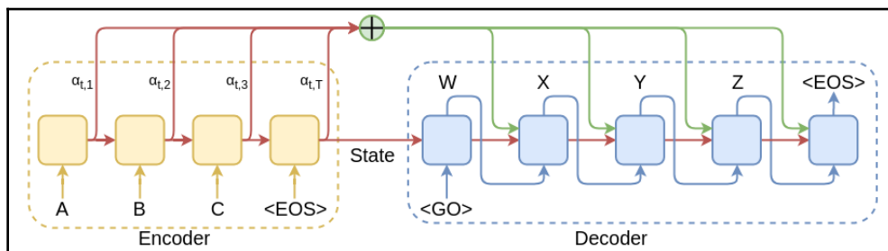
Attention mechanism
