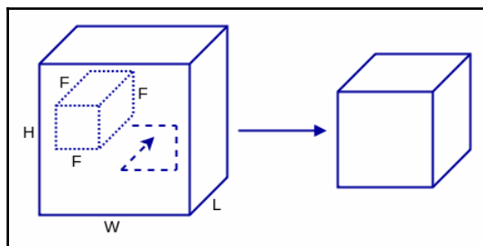
3D convolution
