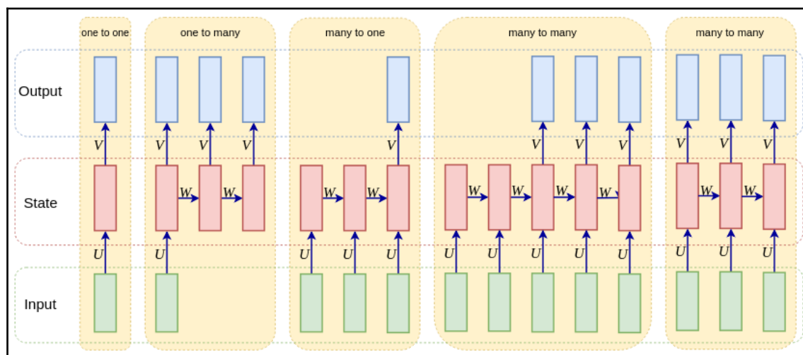
RNN input-output combinations
