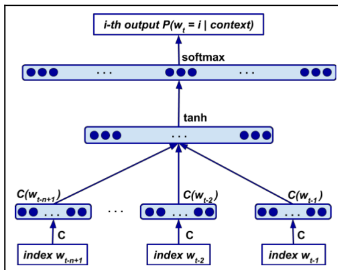
Neural network language model that outputs the probability distribution of the word w_t , given the words w_{t-n+1} \dots w_{t-1} . C is the embedding matrix
