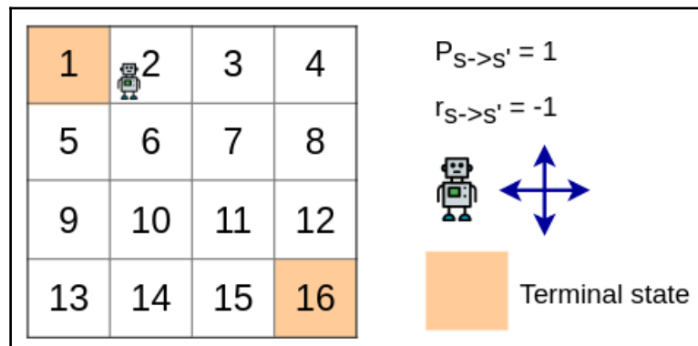
The gridworld environment
