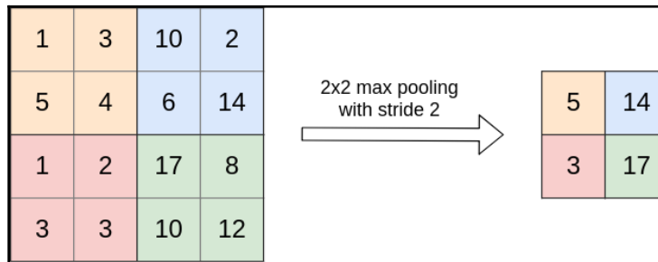
An example of the input and output of a max pooling operation with stride 2 and 2x2 receptive field. This operation discards 3/4 of the input neurons
