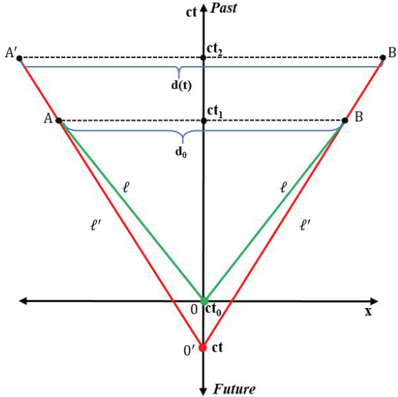
Figure 1.2. A simplified Minkowski diagram imagining a measurement of the distance between the two galaxies ( A and B ) from the observational point of O . 27
