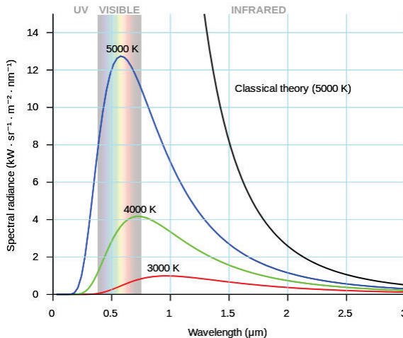
Figure 3.1. Spectral distribution of blackbody radiation as measured (the coloured curves) and theorised by the Rayleigh–Jeans model (the black curve). Planck’s distribution fits into experimental results, while the classical theory doesn’t. The cosmic blackbody radiation shown in figure 1.3 is similar to that of Planck’s in a range of micro-radio wavelengths, giving the CMBR at a low temperature of 2.7 K. 1
