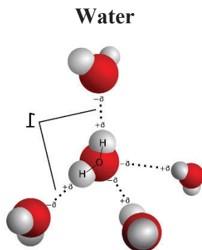
Figure 7.1. An illustration of water molecules having the two H^+ positive ions bonding with the neighbouring negative O^{2-} ion called hydrogen bonding. This kind of bonding between the water molecules gives the extraordinary properties of all phases (vapour, water, and ice). (Licenced under the CC)
