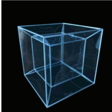
Figure 2.16. 20 Projection of 4D cube (tesseract) in 3D having four dimensions; length, width, height, and additional “trength.”
