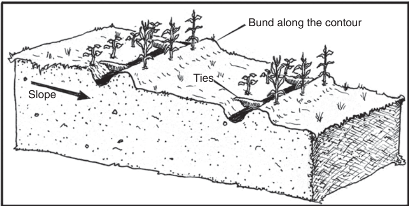
Fig. 7.9. Tied contour ridges.
