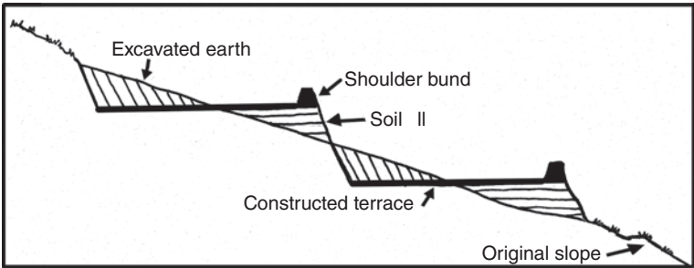
Fig. 7.12. Terrace creation. 28
