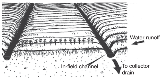
Fig. 11.2. Surface drainage. 38
