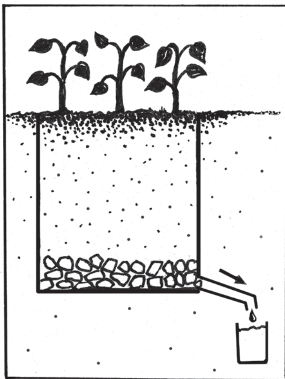
Fig. 4.3. Drainage lysimeter. 6
