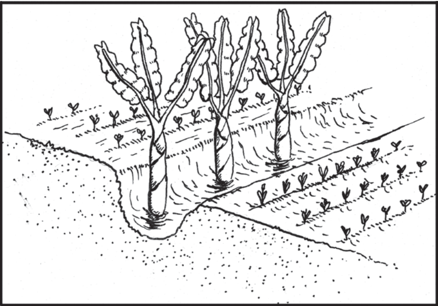
Fig. 7.11. Retention ditches. 25
