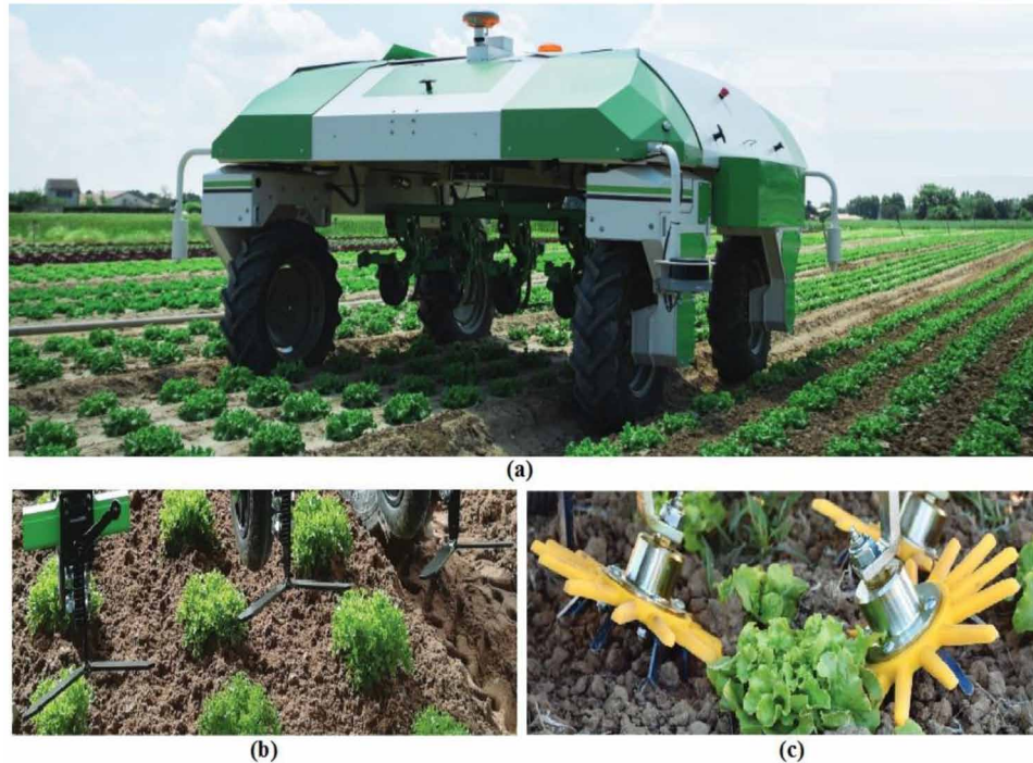
Figure 3. Automated weeding robot for vegetable crops, (a) robot, spiked harrow tool, (rotary hoe) (Preudhomme, 2019).
