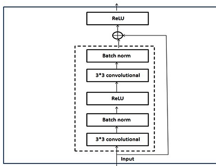
Figure 5. A typical architecture of ResNet
