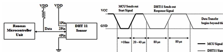
Figure 3. Microcontroller interfacing with DHT11.
