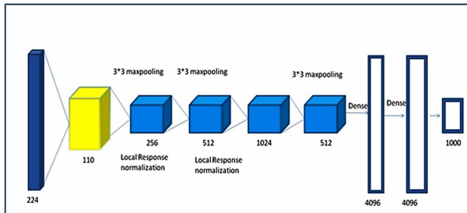
Figure 6. A typical architecture of ZFNet
