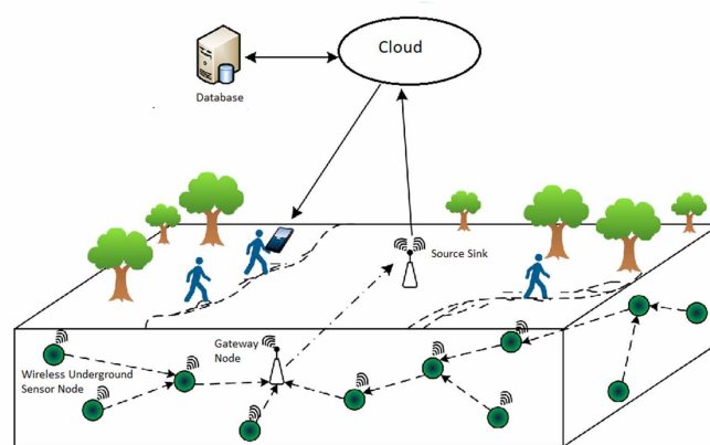
Figure 9. Underground Wireless Sensor Network
