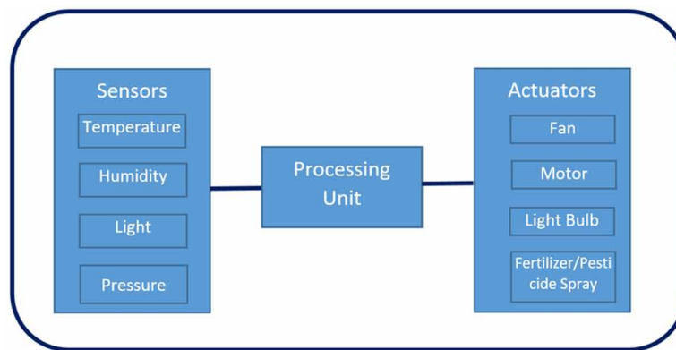
Figure 3. Block Diagram of Smart Greenhouse
