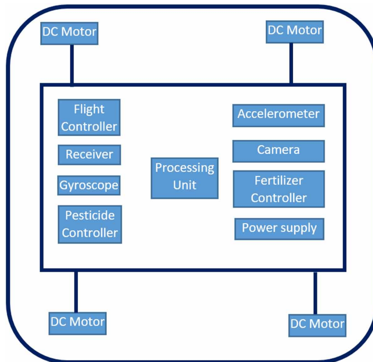
Figure 2. Block Diagram of Unmanned Aerial Vehicle
