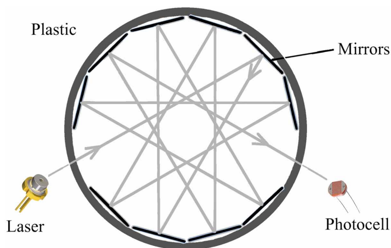
Figure 1. Design of laser scanning application
