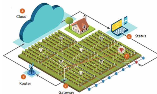
Figure 8. LoRaWAN based Smart Soil Monitoring
