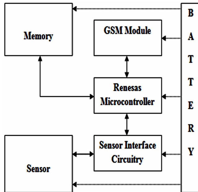
Figure 2. Wireless sensor device architecture
