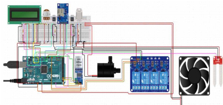
Figure 3. Detailed circuit diagram of the system
