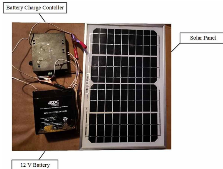
Figure 4. The solar power supply unit
