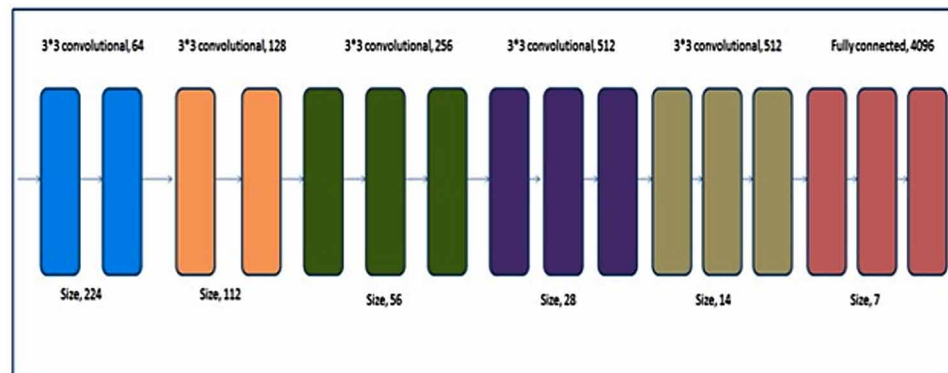
Figure 3. A typical architecture of VGGNet
