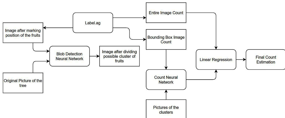
Figure 3. The step-by-step process of counting the fruits using deep learning
