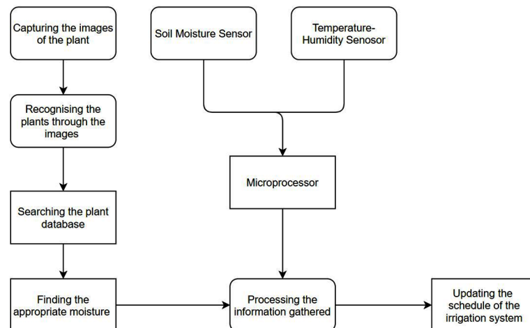
Figure 2. The general process of smart IoT based irrigation system
