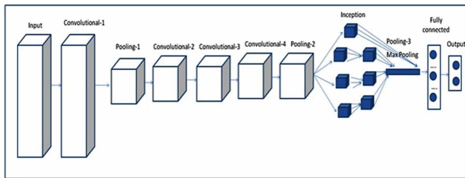
Figure 4. A typical architecture of GoogLeNet
