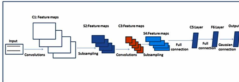
Figure 1. A typical architecture of LeNet5
