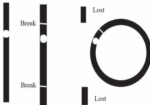
Fig. 12.4 Ring chromosomes.
