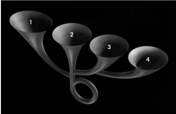
FIGURE 10. Gott-Li self-creating multiverse. The loop at the bottom represents a time machine; the universe gives birth to itself.
