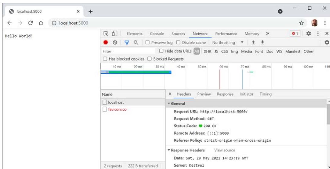
Figure 14.6: Plain text response from http://localhost:5000/
