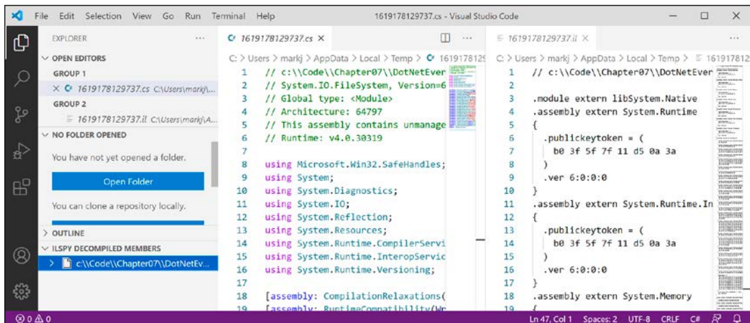
Figure 7.6: Expanding ILSpy DECOMPILED MEMBERS
