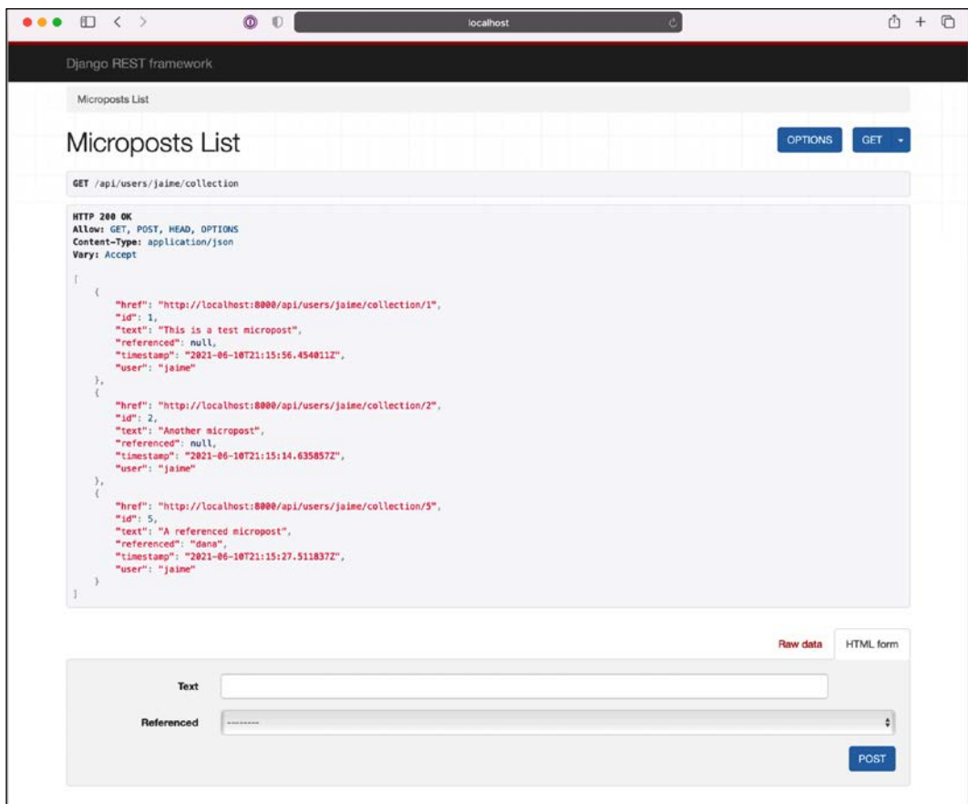
Figure 9.7: Microposts list
