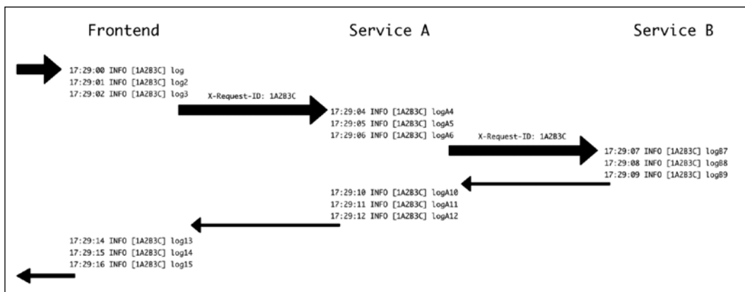
Figure 15.1: Request ID across multiple services
