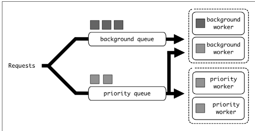
Figure 7.6: Regular worker pulling from multiple queues
