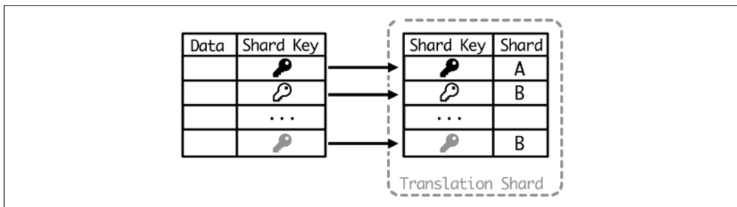
Figure 3.6: Storing shard keys to shards
