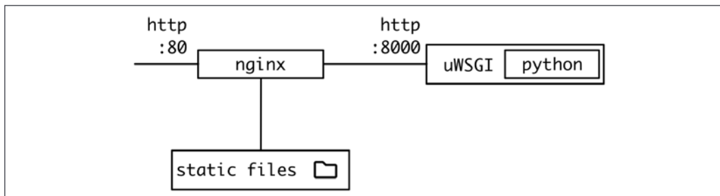
Figure 5.2: Connecting a web server and application server
