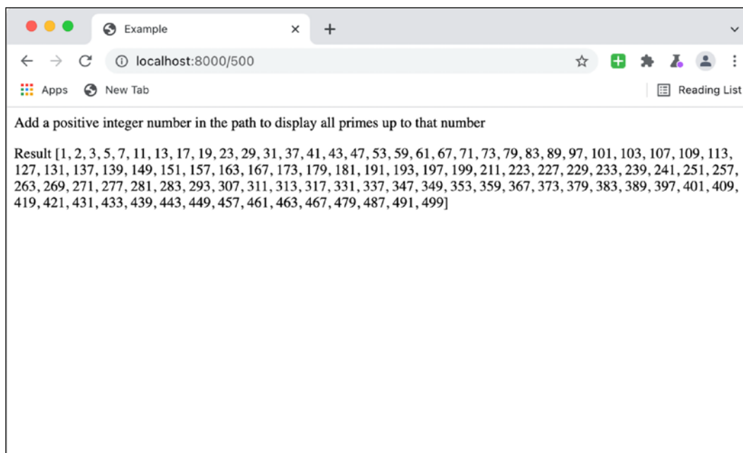
Figure 14.3: The interface displaying all primes up to 500
