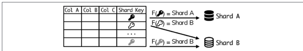
Figure 3.4: Shard keys
