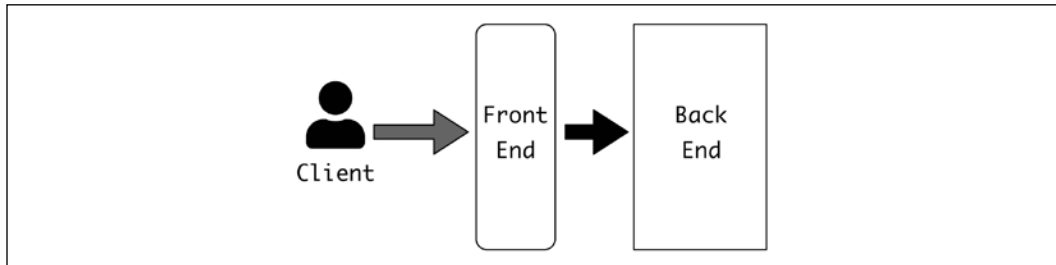
Figure 2.4: Client-Server architecture
