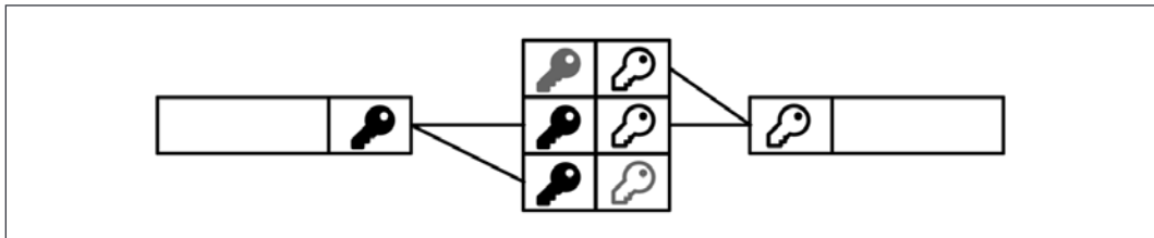
Figure 3.10: Note the intermediary table allows multiple combinations. The first table can reference multiple rows of the second, and the second multiple rows of the first
