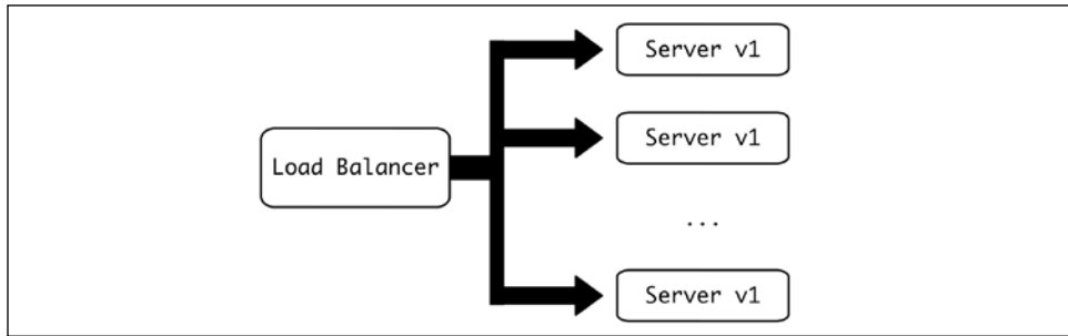
Figure 16.1: Starting point
