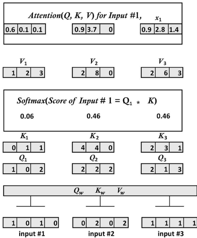
Figure 2.16: Attention representations
