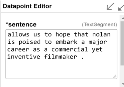
Figure 14.10: Datapoint editor
