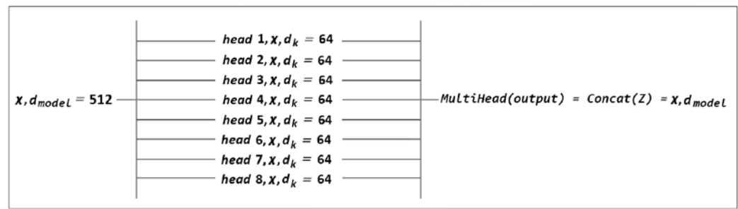
Figure II.1: Multi-head representations
