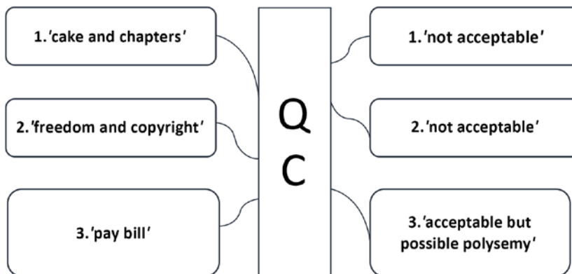
Figure 9.3: Word pairs that tokenizers miscalculated
