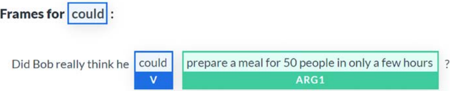
Figure 10.4: Identifying the verb “could” and the argument
