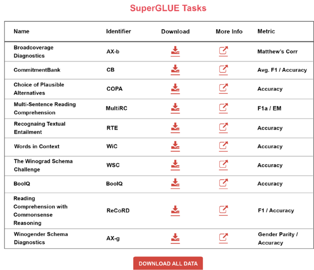
Figure 5.5: SuperGLUE tasks
