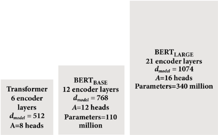
Figure 3.2: Transformer models
