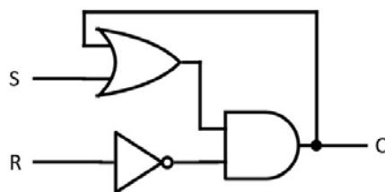
Figure 2.10: SR latch circuit
