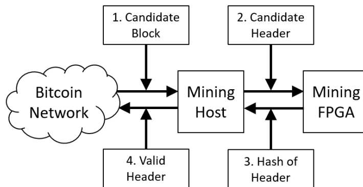
Figure 15.2: Simple FPGA mining configuration
