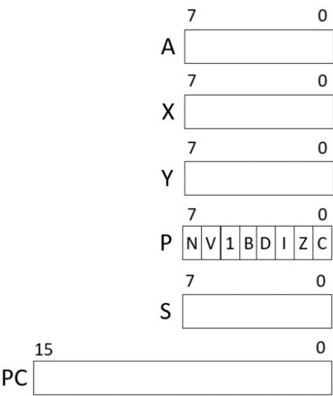
Figure 1.1: 6502 register set
