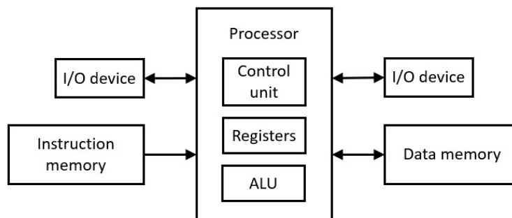
Figure 7.2: Harvard architecture
