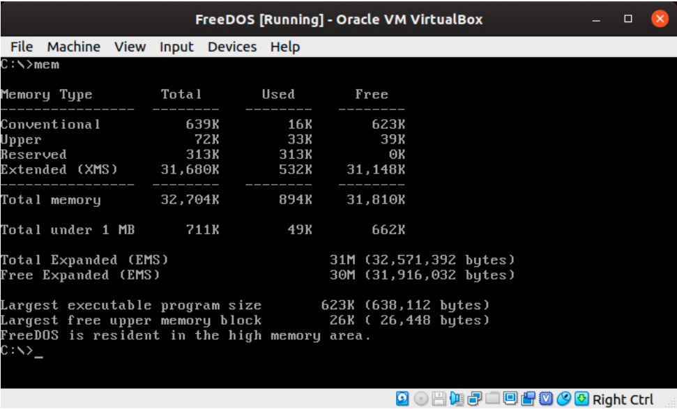
Figure 4: FreeDOS screenshot
